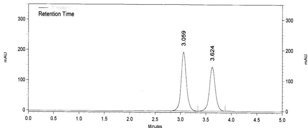
Figure (26): Chromatogram of robustness regarding pH = 5.8
